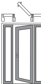
Double Sidelite Right Hand Inswing
